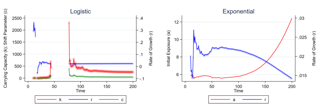
Figure 3: Parameter Estimates Using Simulated Logistic Pandemic
